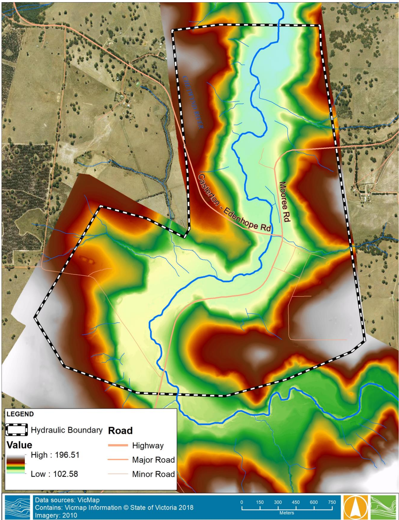
FIGURE 2-21 DIGITAL ELEVATION MODEL
