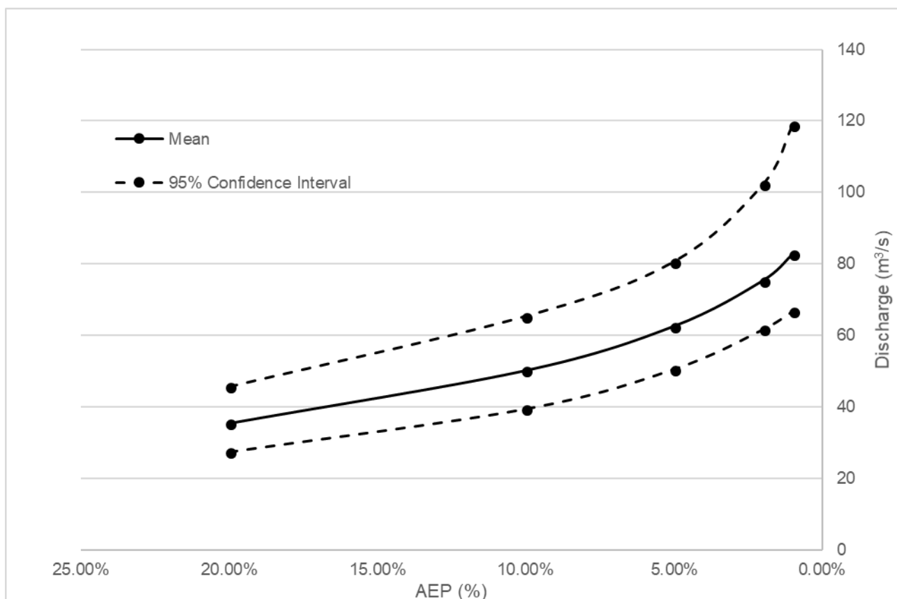
FIGURE 2-14 FLOOD FREQUENCY ANALYSIS RESULTS (1967 – 2016) (AT GAUGE)
