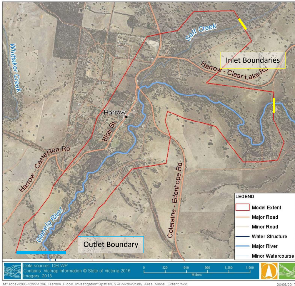
Figure 6-4 Hydraulic model boundaries
