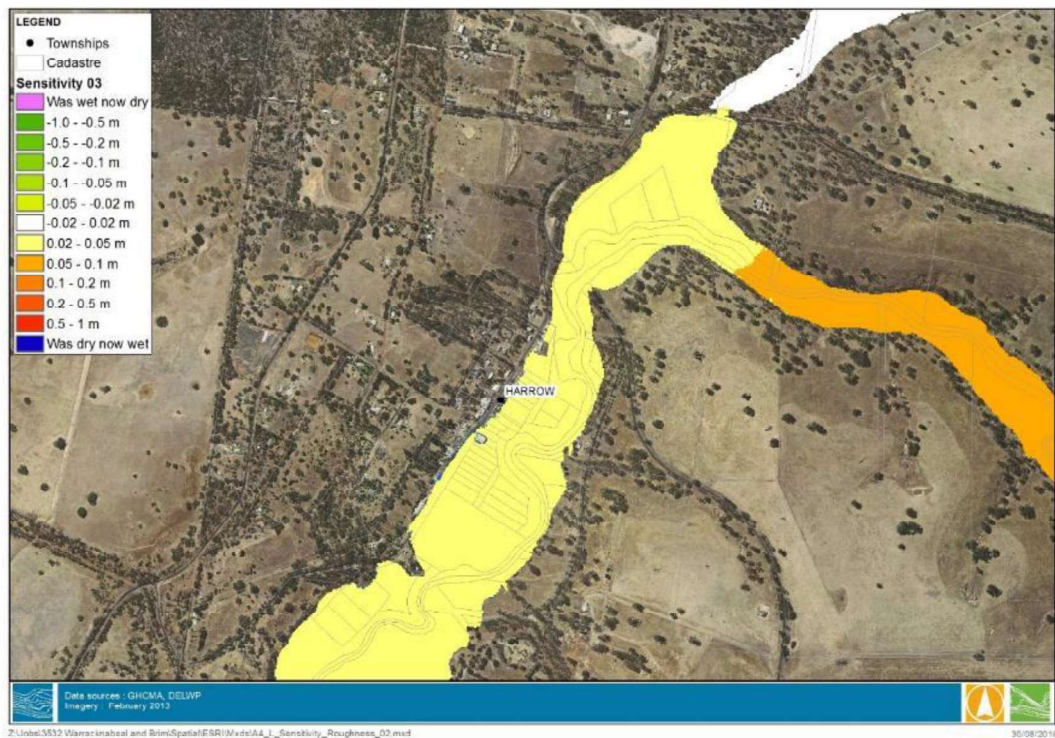
Figure 7-4 Difference in water level due to the 6.9 m 3 /s Rocklands release - Depths at Harrow
