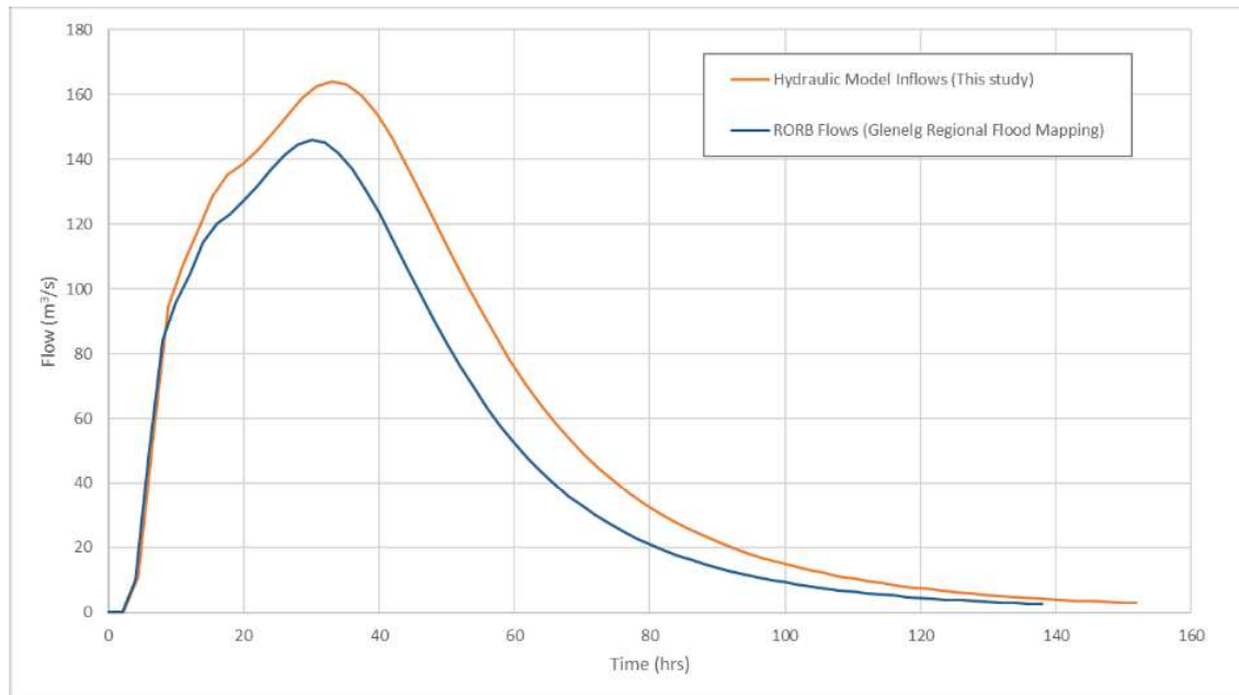
Figure 5-11 Glenelg River at Fulham Bridge 1% AEP design flow hydrographs determined during the Glenelg Regional Flood Mapping Project and this project
