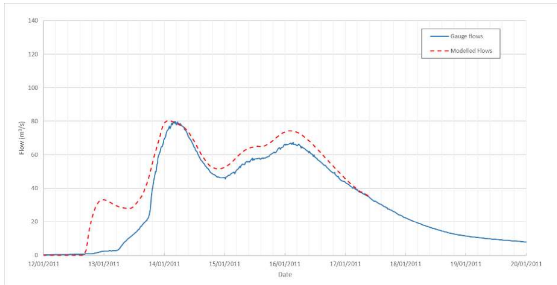
Figure 5-26 January 2011 – Harrow modelled and recorded hydrographs
