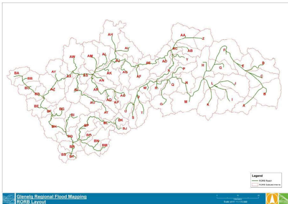
Figure 5-6 Glenelg Regional Flood Mapping RORB Model Structure 1
