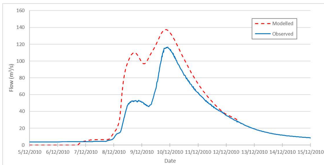
Figure 5-28 December 2010 – Initial loss of 35 mm and continuing loss of 5 mm/hr, 'kc' of 80
