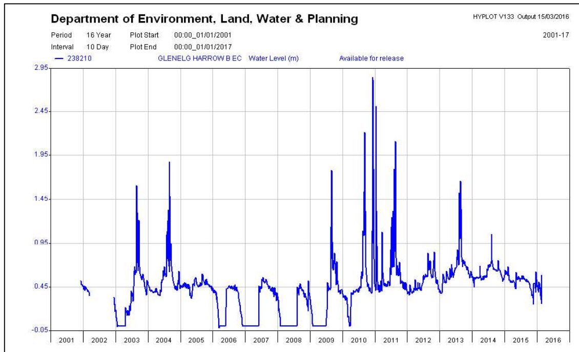
Figure 3-8 Glenelg River at Harrow Gauge Records 2
