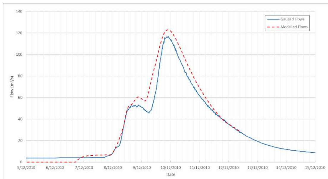
Figure 5-22 December 2010 – Harrow modelled and recorded hydrographs
