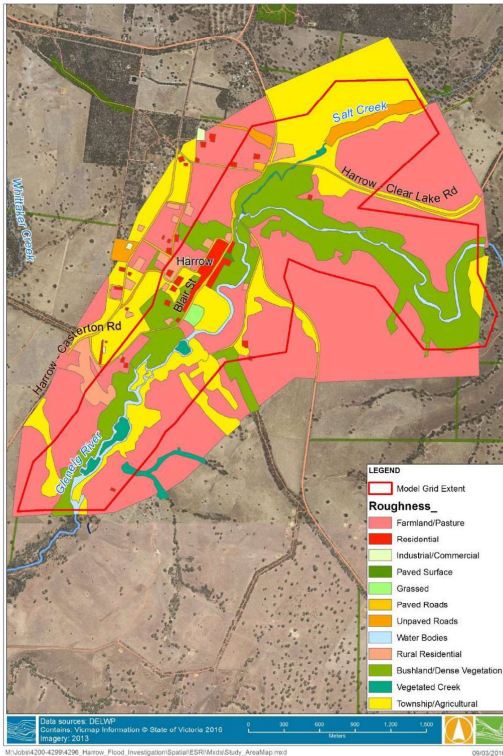
Figure 6-2 Adopted Manning's 'n' roughness values
