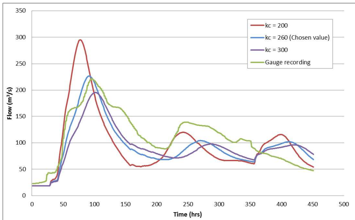
Figure 5-10 Gauged and modelled hydrographs for 'kc' values of 200, 260 and 300 for the 1983 event at Casterton
