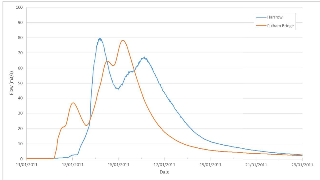
Figure 3-10 January 2011 – Hydrograph comparison at Fulham Bridge and Harrow
