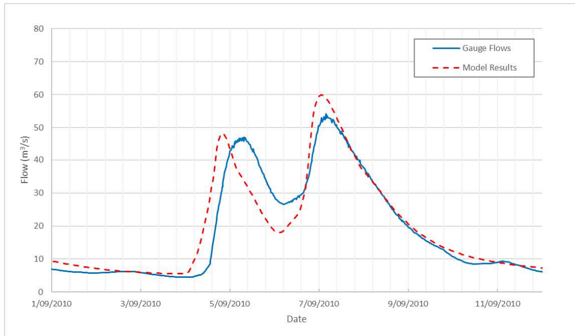
Figure 5-17 September 2010 – Harrow modelled and recorded hydrographs
