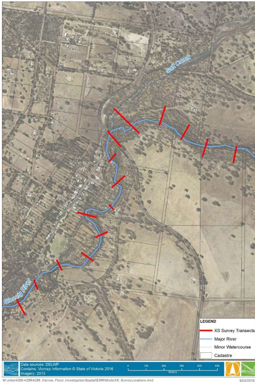
Figure 3-15 Available cross-section survey transects 10
