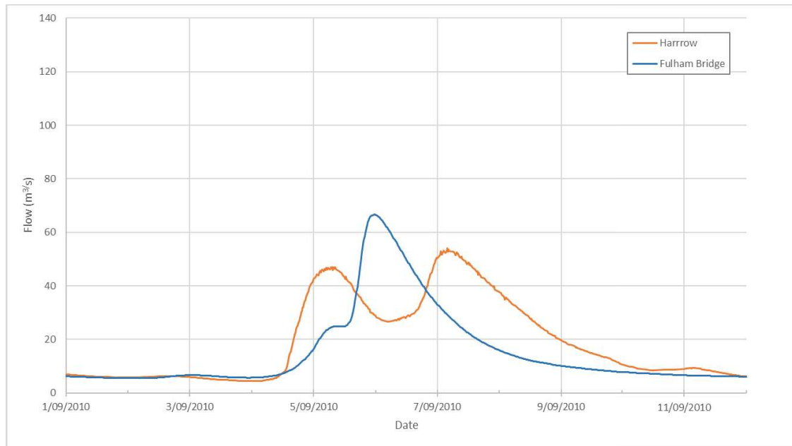
Figure 5-16 September 2010 – Fulham Bridge and Harrow recorded hydrographs
