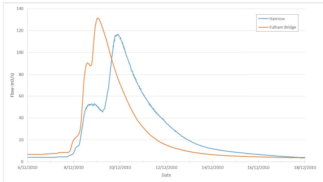
Figure 3-9 December 2010 – Hydrograph comparison at Fulham Bridge and Harrow
